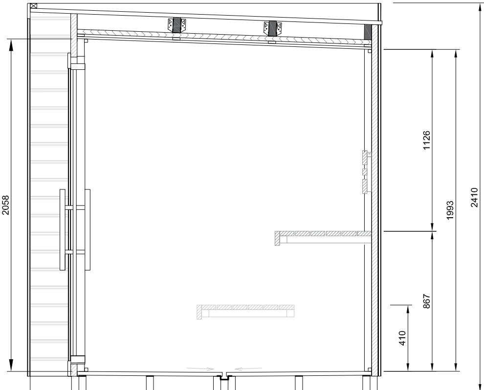
Cross section
