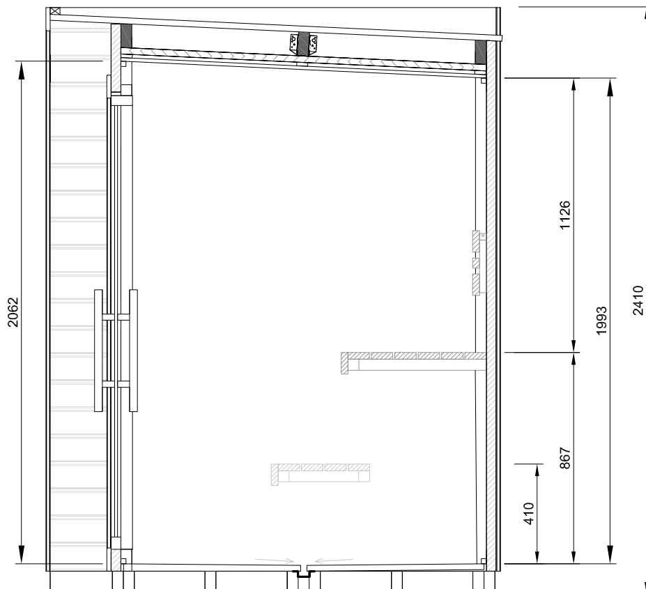
Cross section
